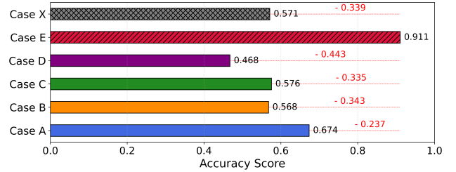
Figure 4. Cross-dataset domain adaptation performance of ViLT. Case A: Train on NHMC, Test on IIMC (at genus); Case B: same as A (at species); Case C: Train on BeetlePalooza, Test on IIMC (at genus); Case D: same as C (at species); Case E: Train on NHMC, Test on BeetlePalooza (at genus); Case X: Average of Cases A, B, C, and D. Cases A to D represent lab-to-in-situ domain shifts for both genus and species levels, while Case E is evaluated at the genus level only due to limited species-level overlap between NHMC and BeetlePalooza.
